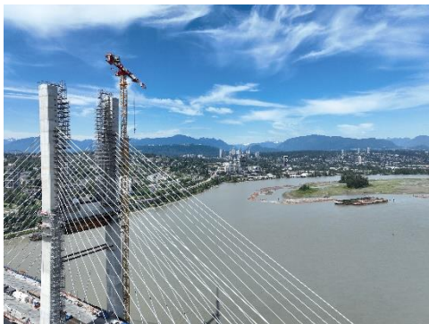
Figure 3: Stay cable installation continues.
