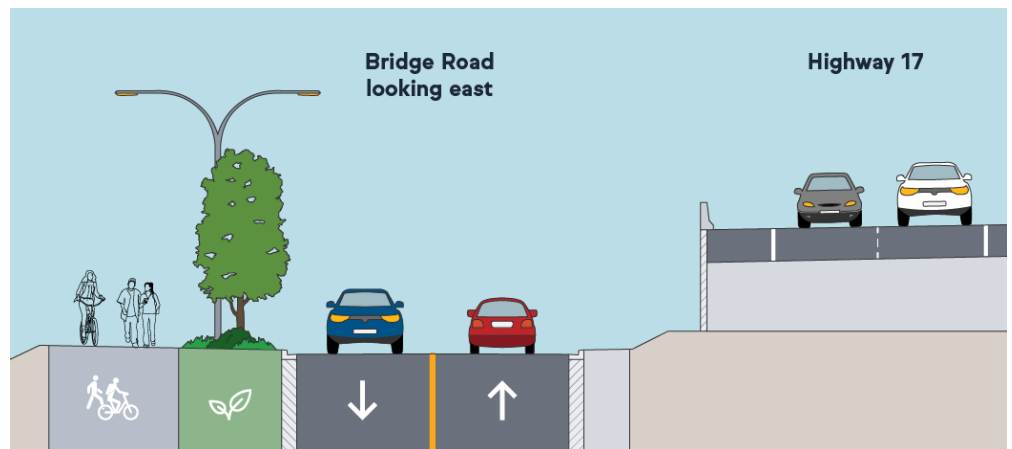
Cross-section illustration of two-way Bridge Road in Surrey.
