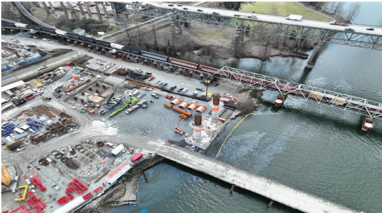
FIGURE 2 – AERIAL OF S2 COLUMN CONSTRUCTION
