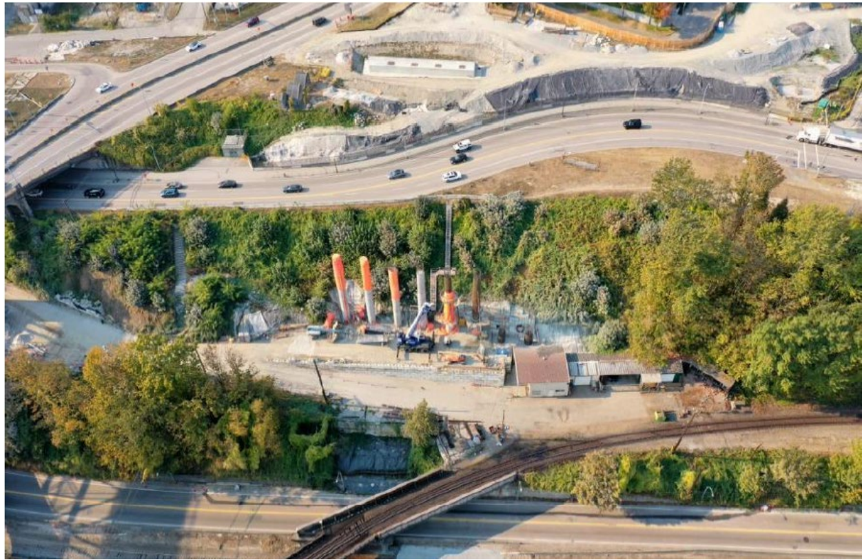
FIGURE 4 – PIER N2 COLUMN INSTALLATION (FRONT) AND N3 ABUTMENT WORK (BACK)
