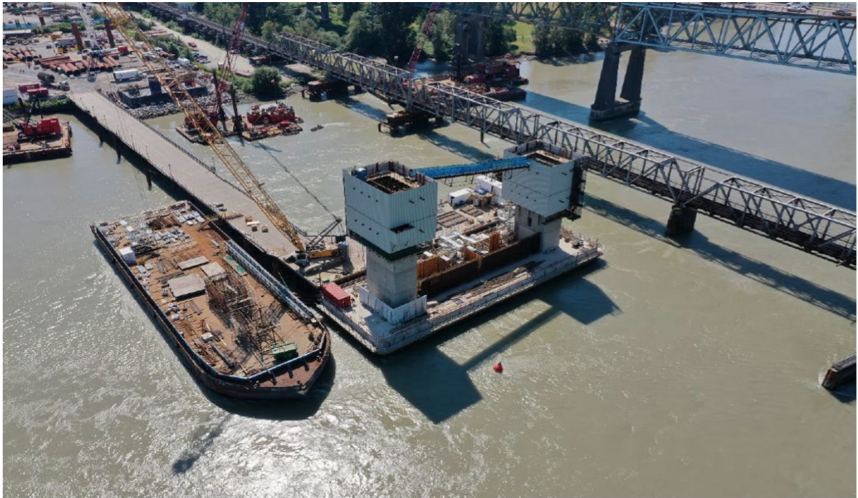
FIGURE 1 – PROGRESS OF THE S1 TOWER CONSTRUCTION
